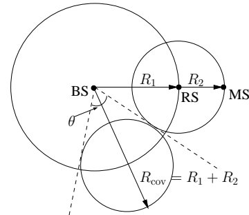
Fig. 2. Illustration of the definition of coverage radius R_{cov} for the relay-assisted cellular system. Also shown is the method to evaluate the angle \theta subtended by each RS at the BS. \theta = \sin^{-1}(R_2/R_1) .
