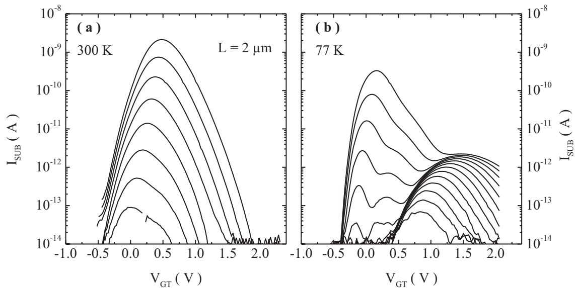
Figure 5.6: I_{SUB} vs V_G characteristics of a LAC device of L = 2 \mu\text{m} , (a) at 300 K for V_D = 1.8 to 2.5 V with \Delta V_D = 0.1 V, and (b) at 77 K for V_D = 1.3 to 2.5 V with \Delta V_D = 0.1 V.
