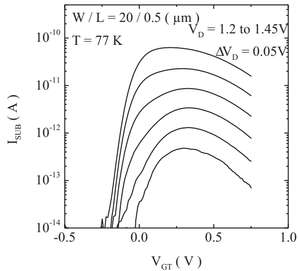
Figure 4.5: I_{SUB} vs V_G characteristics at 77 K near bandgap voltages in n-channel MOSFET of L = 0.5 \mu m .
