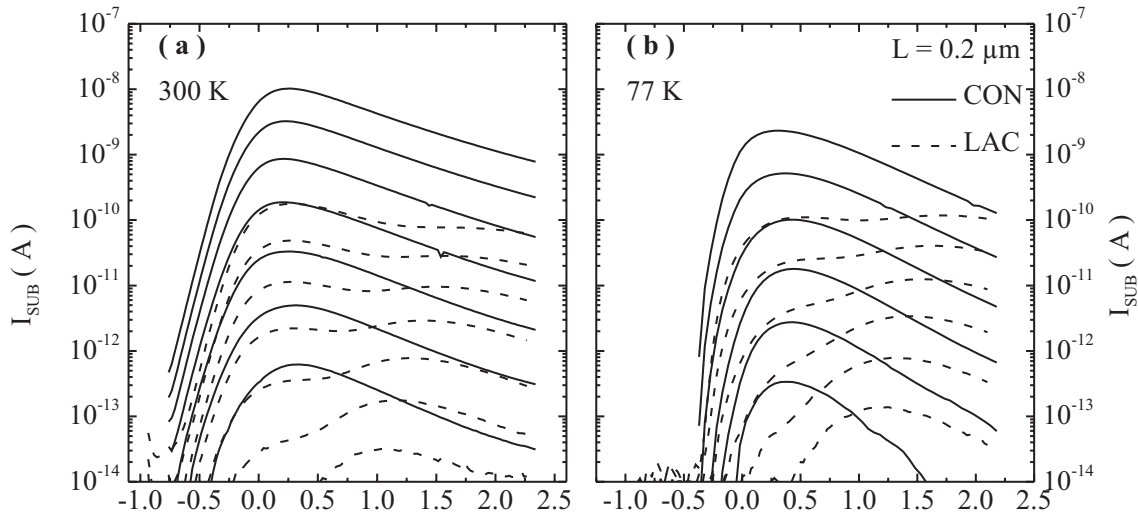
Figure 5.25: Comparison of I_{SUB} vs V_G data of CON and LAC devices of L = 0.2 \mu\text{m} : (a) at 300 K, V_D = 0.9 to 1.5\text{V} and (b) at 77 K, V_D = 1 to 1.5\text{V} . \Delta V_D = 0.1\text{V} . The LAC device was operated in the forward mode.
