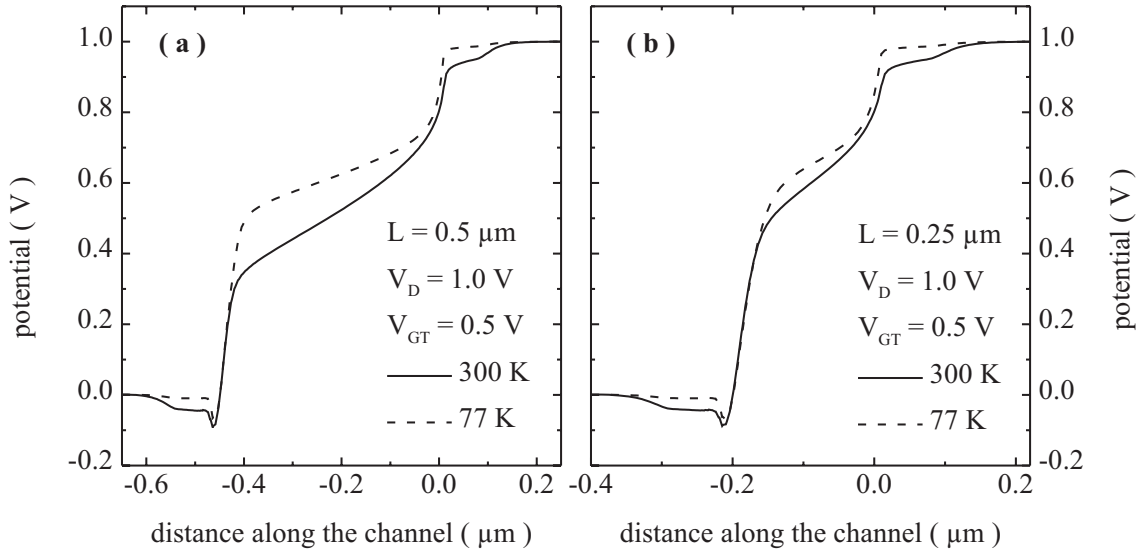
Figure 5.32: Temperature Dependence of the potential profile for (a) 0.5 \mu\text{m} and (b) 0.25 \mu\text{m} LAC devices in the forward mode. The profiles shown are for a cutline 1 nm below the interface. Drain junction is taken as the reference.
