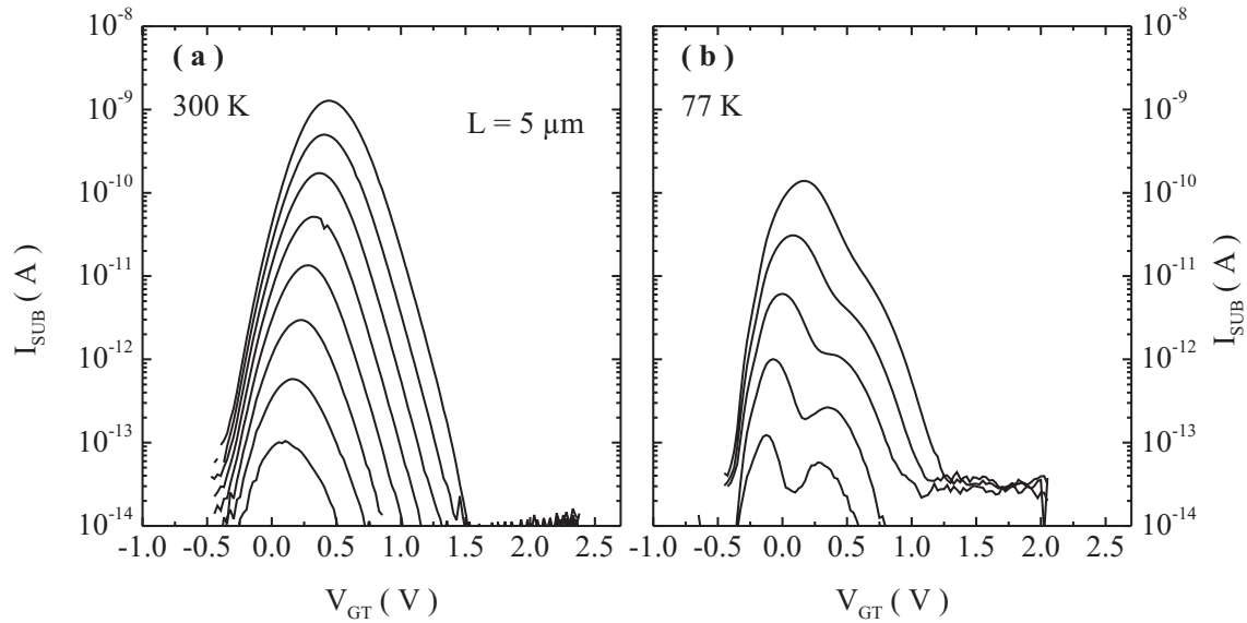
Figure 5.5: I_{SUB} vs V_G characteristics of a LAC device of L = 5 \mu\text{m} , (a) at 300 K for V_D = 1.8 to 2.5 V with \Delta V_D = 0.1 V, and (b) at 77 K for V_D = 2.1 to 2.5 V with \Delta V_D = 0.1 V.
