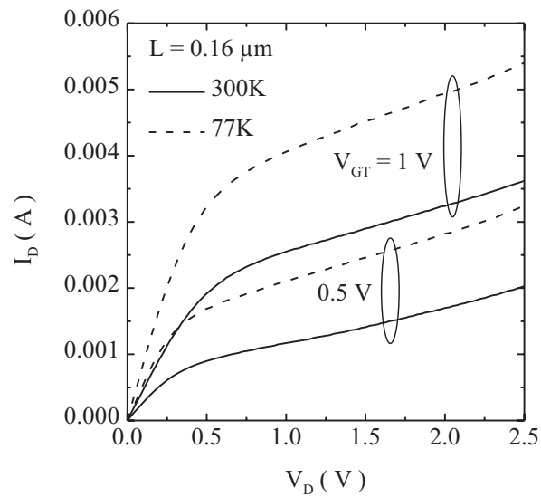
Figure 3.2: Measured output characteristics of devices of channel length 0.16 \mu\text{m} and width 10 \mu\text{m} at 300 and 77 K.
