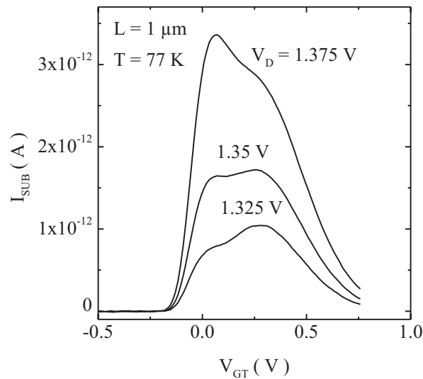
Figure 4.6: I_{SUB} vs V_G characteristics at 77 K near bandgap voltages in n-channel MOSFET of L = 1 \mu m . The y-axis is linear.
