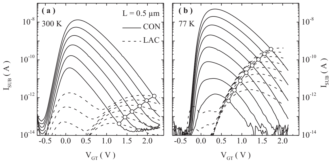
Figure 5.26: Comparison of I_{SUB} vs V_G data of CON and LAC devices of L = 0.5 \mu\text{m} : (a) at 300 K, V_D = 1.3 to 1.8\text{V} in 0.1\text{V} steps, and (b) at 77 K, V_D = 1.3 to 2\text{V} in 0.1\text{V} steps. The LAC device was operated in the forward mode. The circles represent the points of intersection of the plots for the CON and LAC for identical V_D . For V_{GT} to the right of the intersections, the I_{SUB} for LAC is larger.
