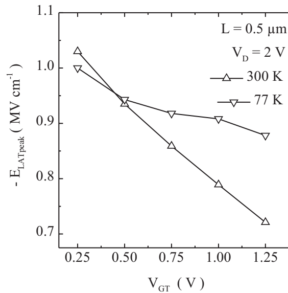
Figure 3.12: E_{LATpeak} , at a depth of 1 nm from the interface for a device of channel length 0.5 \mu\text{m} , versus V_{GT} at 300 and 77 K. The peak field decreases as V_{GT} is increased.
