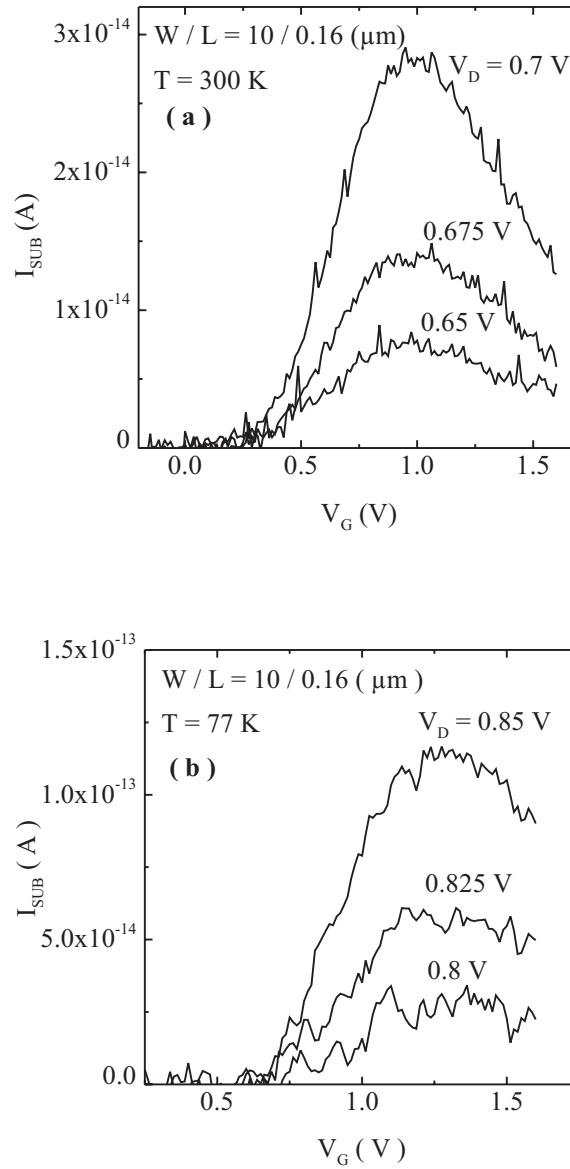
Figure 4.1: Bell shaped I_{SUB} vs V_G characteristics, a signature of impact ionization in MOSFETs, measured for n-channel devices of L = 0.16 \mu\text{m} . (a) at 300 \text{ K} and (b) at 77 \text{ K} . Impact ionization is observed for V_D of 0.65 \text{ V} at 300 \text{ K} and 0.8 \text{ V} at 77 \text{ K} . These voltages are much below the bandgap voltages of silicon at either temperature.
