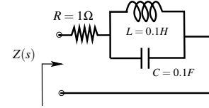
Fig. 1. A controllable RLC circuit
