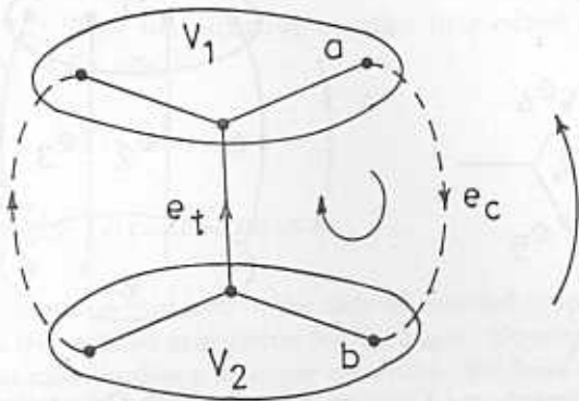
Figure 3.7: Relation between f-circuit and f-cutset
