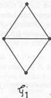
Figure 3.9: Cyclically Connected and Cyclically Disconnected Graphs
