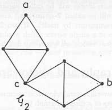
Figure 3.9: Cyclically Connected and Cyclically Disconnected Graphs
