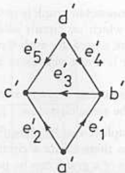
Figure 3.8: Isomorphic Directed Graphs
