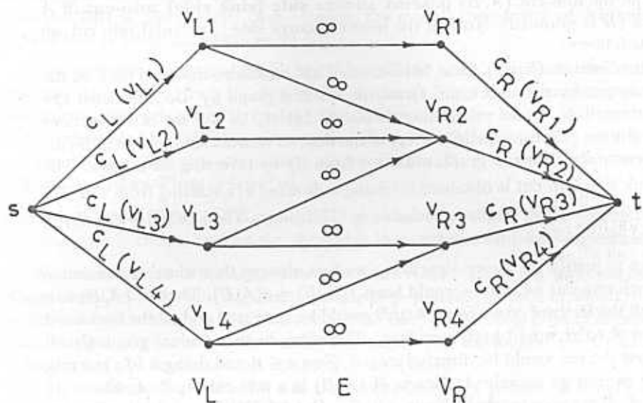
Figure 3.13: The Flow Graph associated with B
