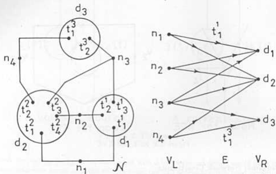
Figure 5.2: An Electrical Network \mathcal{N} and its Bipartite Graph Representation
