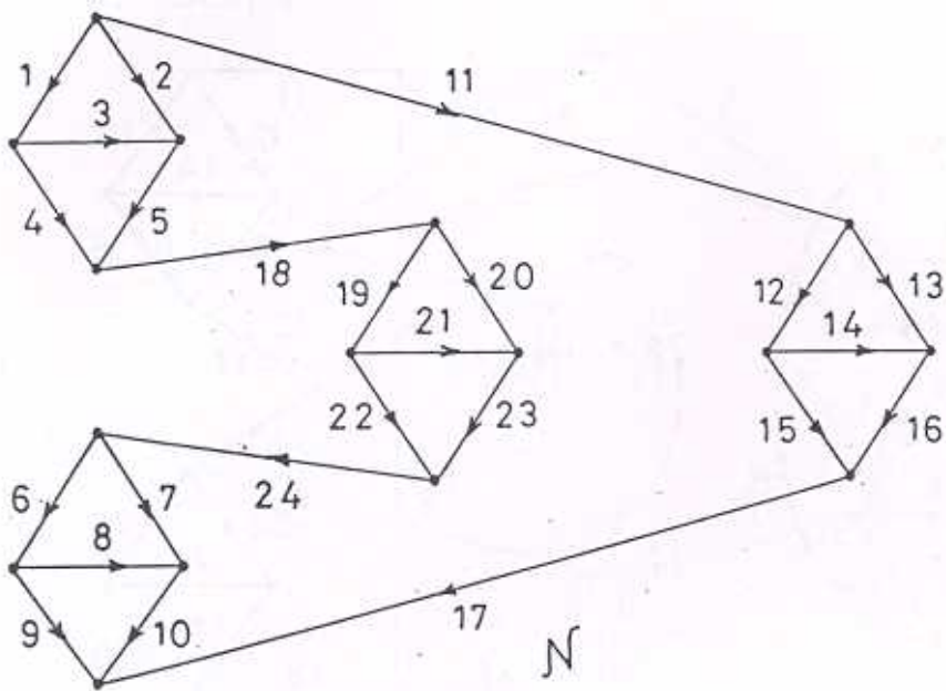
Figure 1.2: A Network to be decomposed into Multiports
