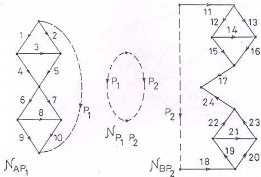
Figure 1.3: Decomposition into Multiports
