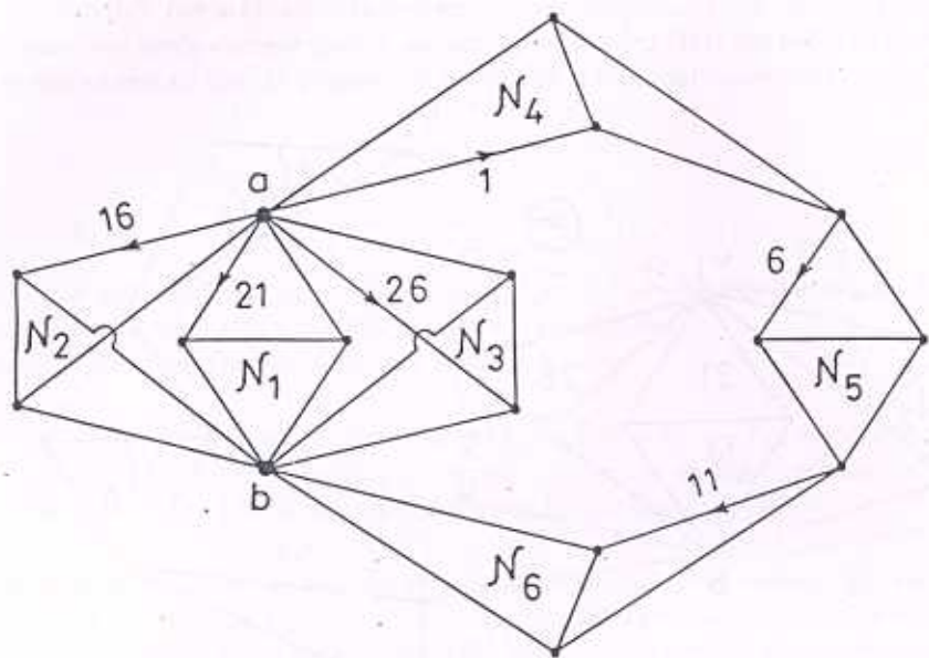
Figure 1.4: Network \mathcal{N} to Illustrate the Fusion-Fission Method
