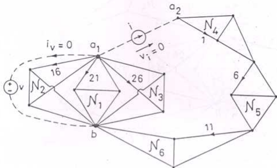
Figure 1.5: A Network equivalent to \mathcal{N} with Virtual Sources.
