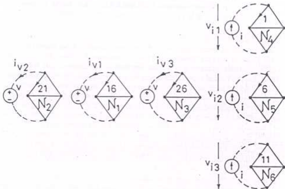
Figure 1.6: Network \mathcal{N} decomposed by the Fusion-Fission Method
