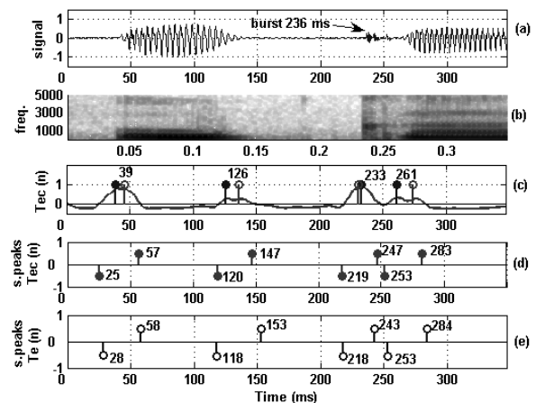
Fig. 3. Processing results for /uka/ : Waveform(a), spectrogram (b) transition index T_{ec} (c), and transition segment boundaries using T_{ec} (d), and using T_e (e).
