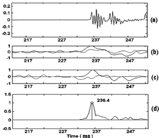
Fig. 4. (a) Windowed segment used in second pass, (b) energy and ZCR ROR's of level 1, (c) ROR's of level 2, and (d) transition index T_{ez} computed from ROR's in (b) and (c).
