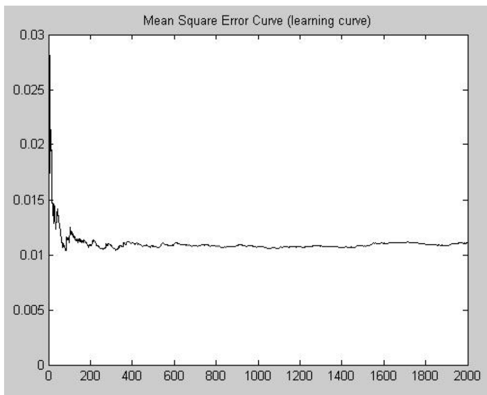
Fig 4. mean square error for RLS
