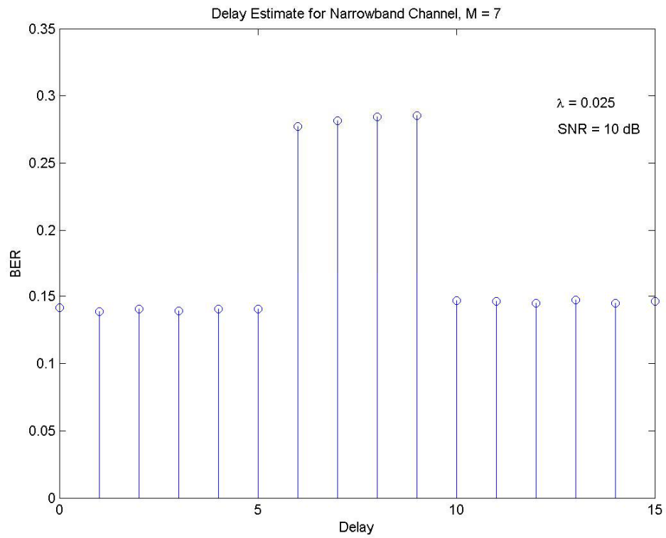
Fig 1: delay estimate for narrow band channel
