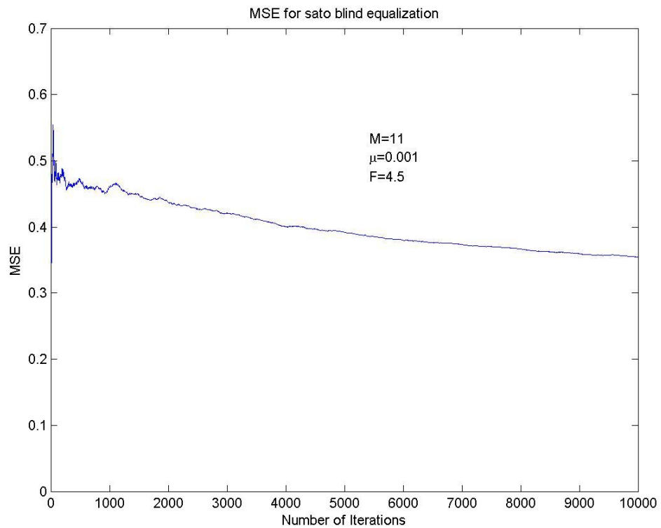
Fig 2: mean square error curve for sato's algorithm
