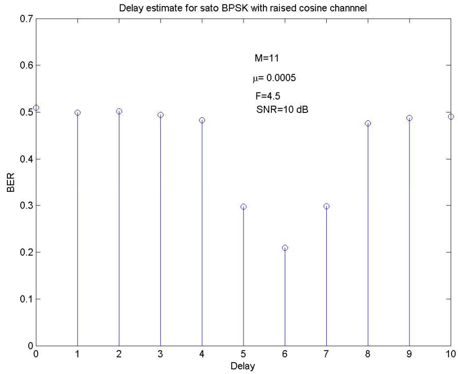
Fig 1: delay estimate for sato blind equalizer
