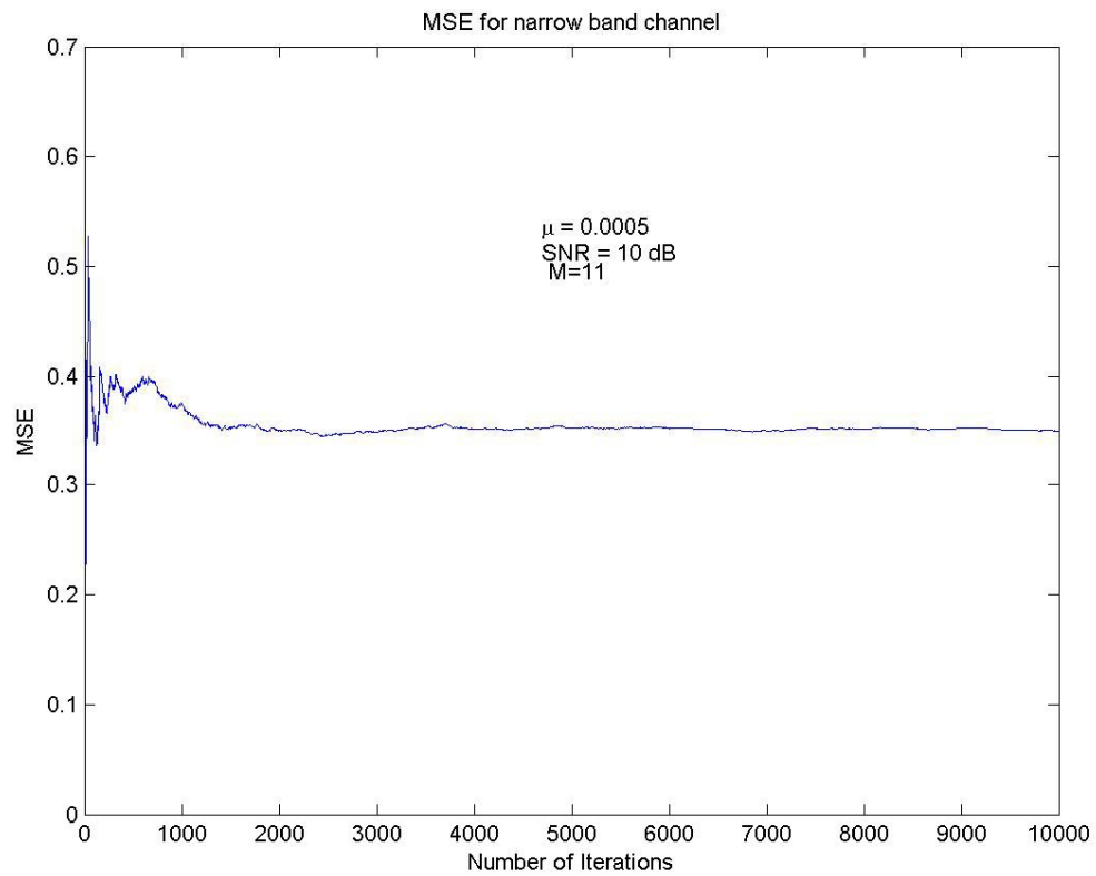
Fig 4: mean square error curve for narrow band channel.
