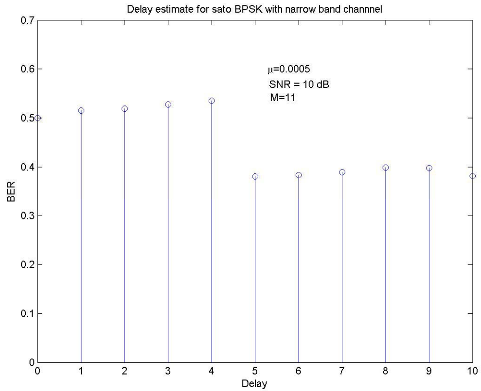
Fig 3: delay estimate for sato's blind equalizer for narrow band channel
