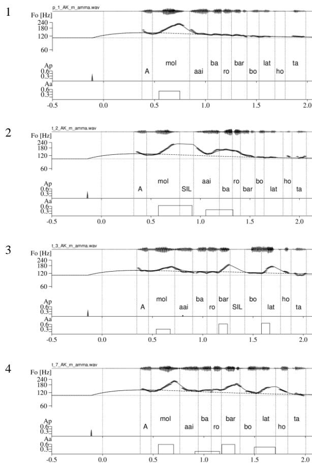
Figure 3: Speech waveform, F0 contour and underlying Fujisaki model parameters for 'Amol aai barobar bolat hota' - (top to bottom) foci: (1) narrow on Amol, (2) narrow on aai, (3) narrow on bolat, and (4) broad.
