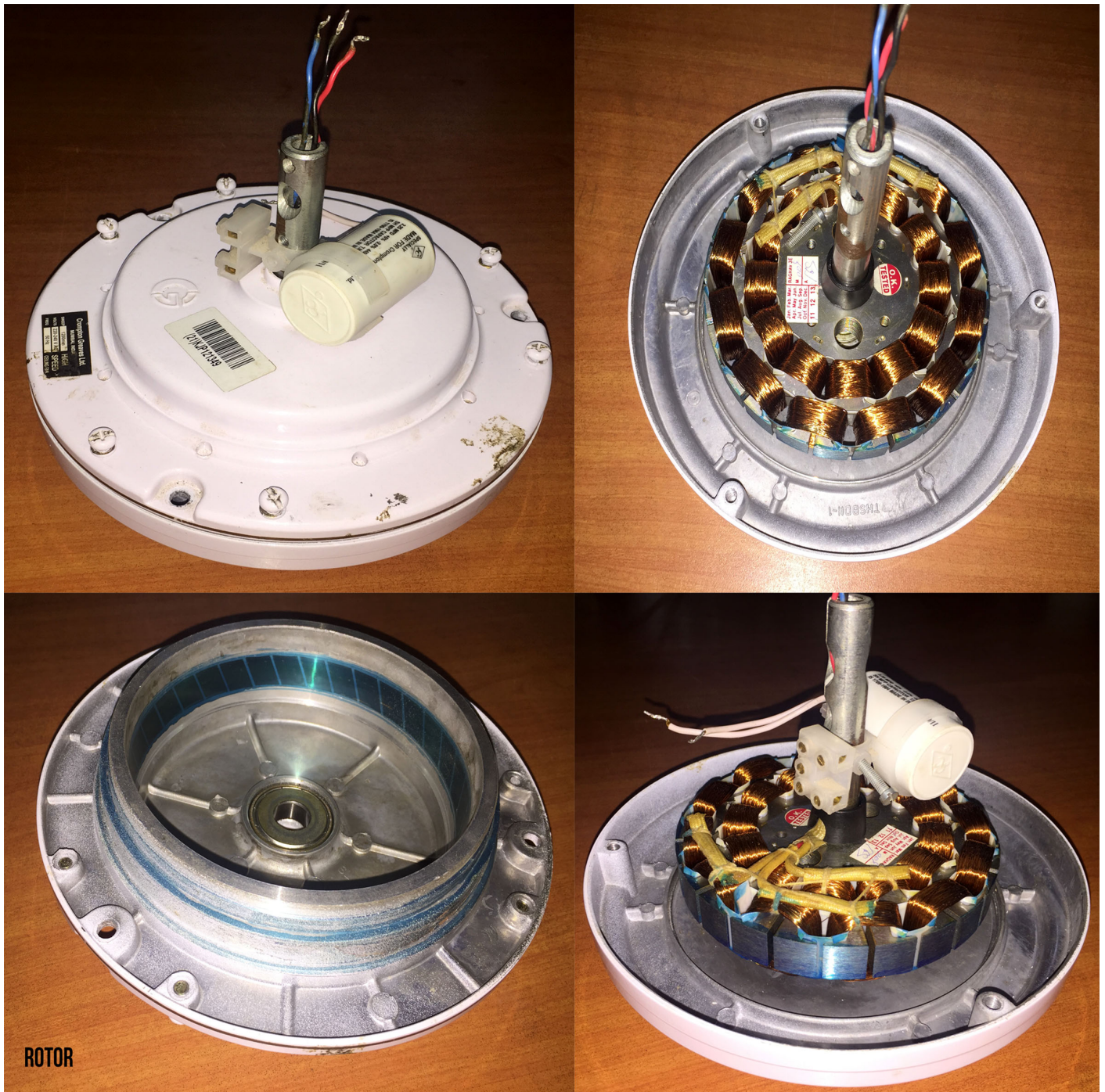
Figure 1: Single Phase Induction Motor used in a residential Fan
