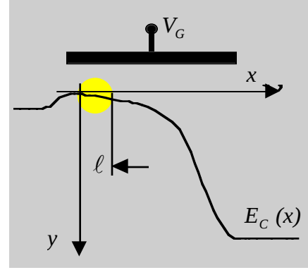
Fig. 1 The conduction band edge vs. position from the source to the drain of a nanoscale MOSFET under high gate and drain bias.
