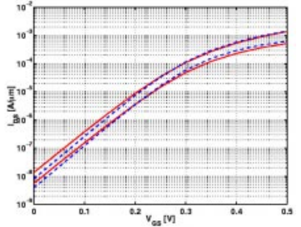
Fig. 7 The \log(I_D) vs. V_{GS} characteristics of the 10nm DG SOI MOSFET as computed by a classical (dashed) and quantum mechanical (solid) simulation for V_D = 0.05 and 0.5V.
