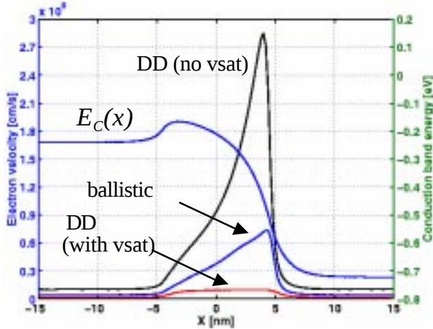
Fig. 9 Average velocity vs. position at V_G = V_D = 0.5V for the 10 nm DG SOI-MOSFET. For reference, we also show the conduction band profile; the beginning of the channel is at the top of the barrier.
