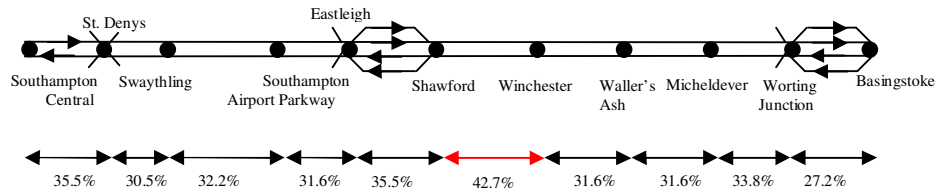
Figure 6 - Timetable compression according to the CUI method.
