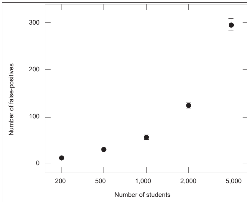
Figure 5: Demonstration of 90% band of false-positives for nQ = 30 and different nS for 10% cut-off
