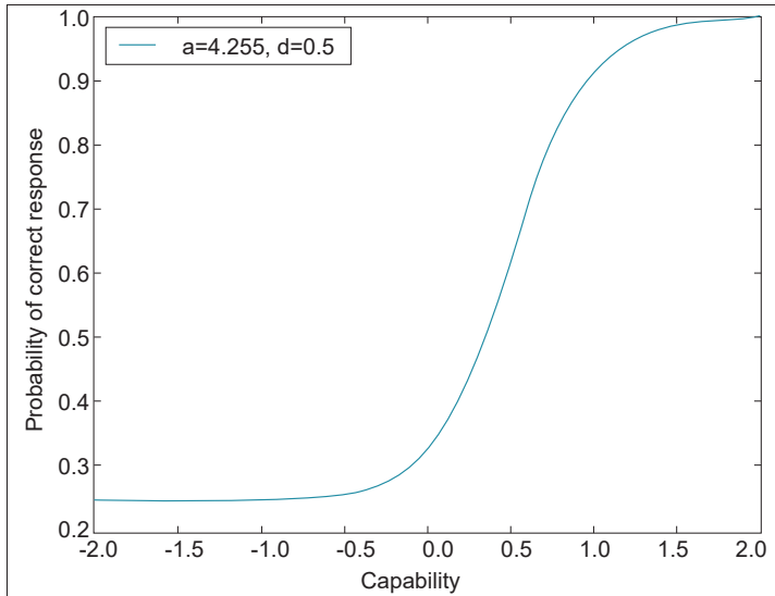
Figure 1: ICC for correct response with d = 0.5 , a = 4.255 and g = 0.25
