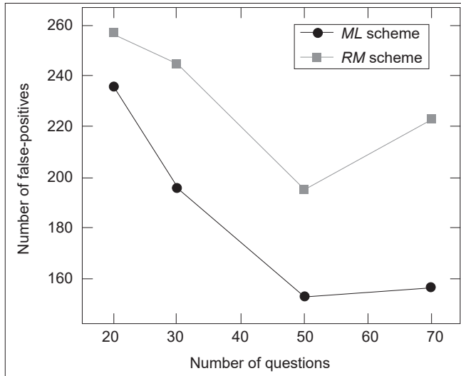
Figure 10: Number of gate-crashers for nS=2000 and different nQ for 30% cut-off
