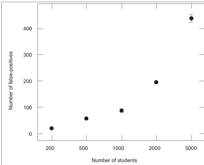
Figure 7: Demonstration of 90% band of gate-crashers for nS = 2000 and different nQ for 30% cut-off
