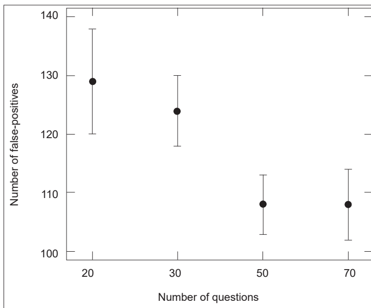
Figure 9: Demonstration of 90% band of gate-crashers for nS= 2000 and different nQ for 10% cut-off
