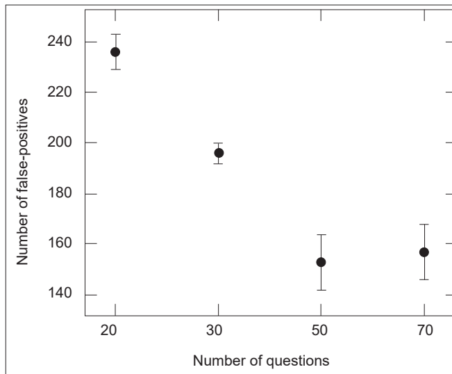
Figure 11: Demonstration of 90% band of gate-crashers for nS = 2000 and different nQ for 30% cut-off
