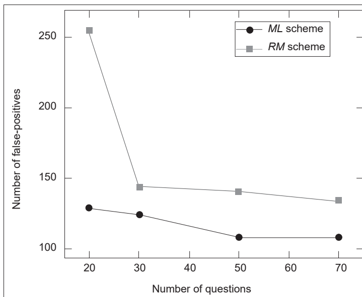
Figure 8: Number of gate-crashers for nS= 2000 and different nQ for 10% cut-off
