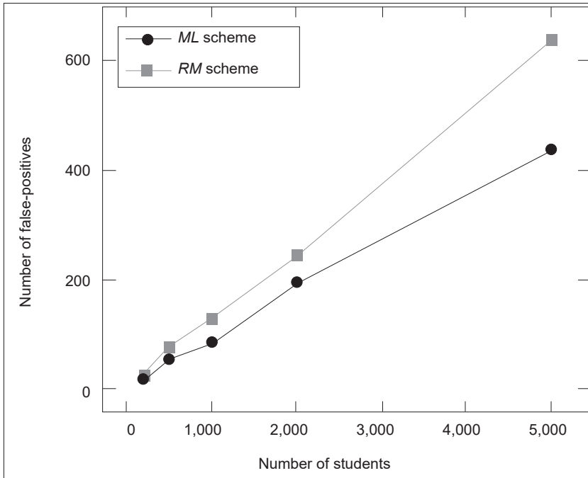
Figure 6: Number of false-positives for nQ = 30 and different nS for 30% cut-off
