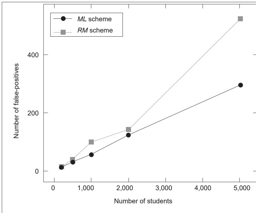
Figure 4: Number of false-positives for nQ = 30 and different nS for 10% cut-off
