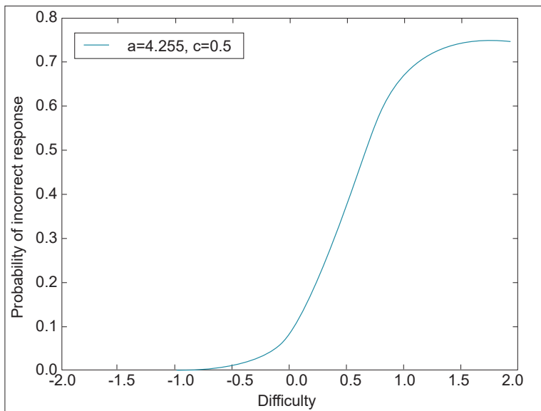
Figure 2: ICC for incorrect response with c = 0.5 , a = 4.255 and g = 0.25
