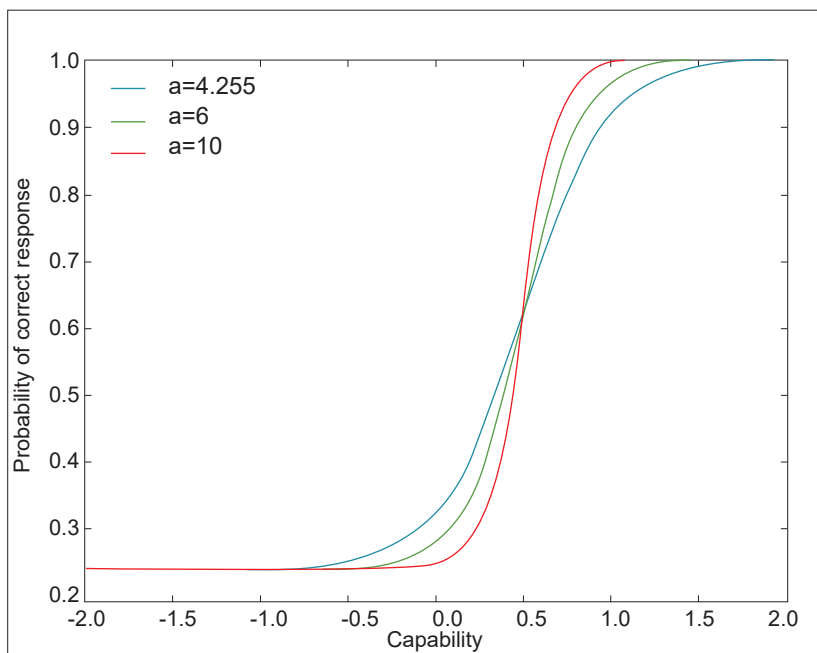
Figure 3: ICC for correct response with d = 0.5 and g = 0.25
