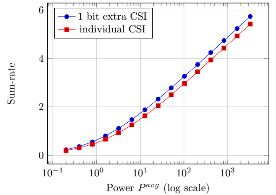
Fig. 2. Sum-rate improvement by additional CSI
