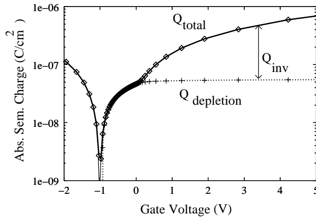
Figure 6: Semiconductor charge as a function of gate voltage
