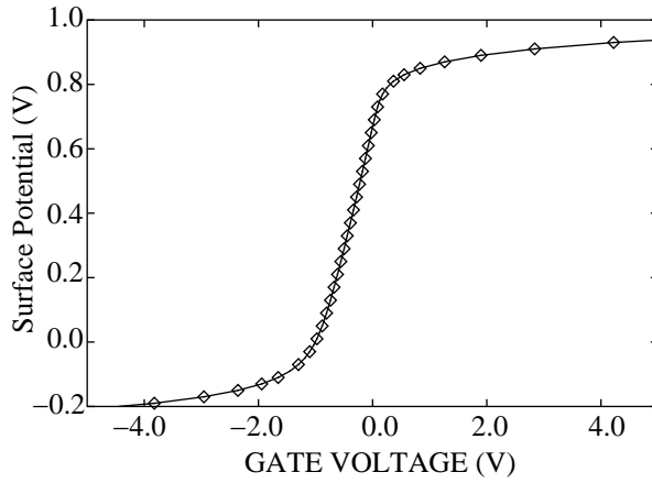
Figure 5: Surface potential as a function of gate voltage
