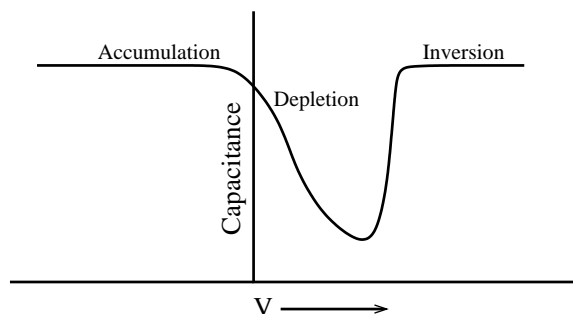
Figure 3: Low frequency capacitance for a MOS capacitor
