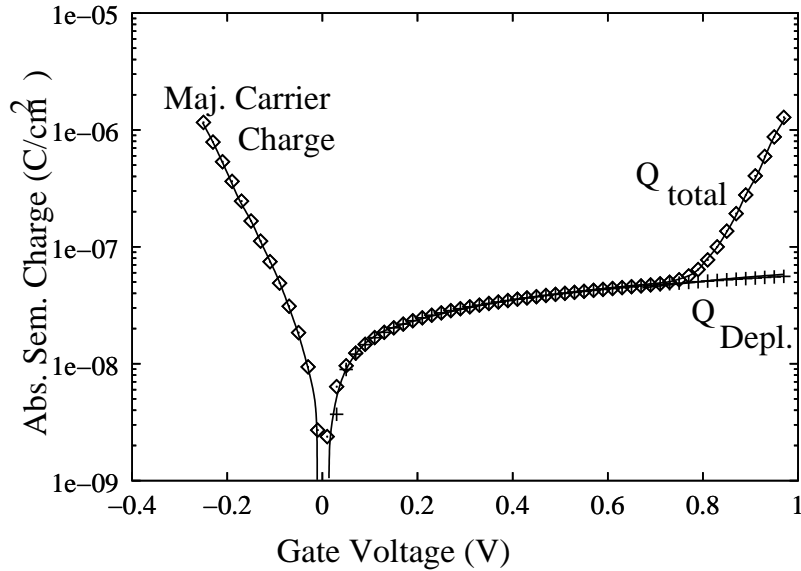
Figure 4: semiconductor charge as a function of surface potential
