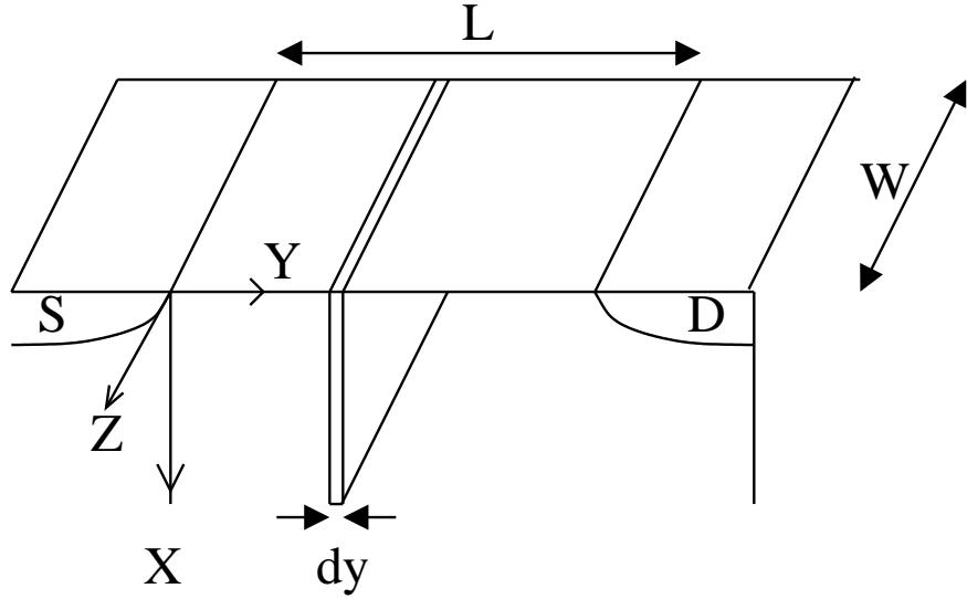
Figure 8: Coordinate system used for analysing the MOS transistor
