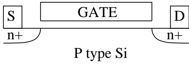
Figure 7: A MOS Transistor
