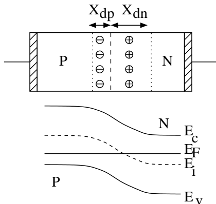
Figure 2: The abrupt p-n junction
