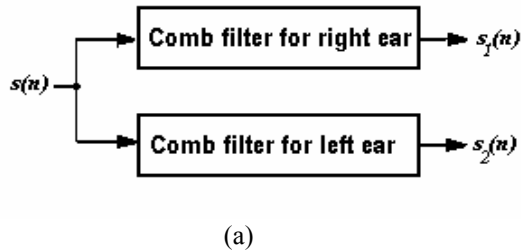
Figure 1: Spectral splitting (SS): (a) Schematic, (b) magnitude response of the comb filter pair, S.R. = 10 k Sa/s, pass band ripple < 1 dB, stop band attenuation > 30 dB, = 78 - 117 Hz transition width
