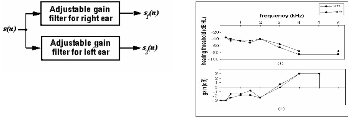
Figure 4: Adjustable gain filter (AG): (a) schematic, (b) pure tone audiogram of a subject and the corresponding magnitude responses
