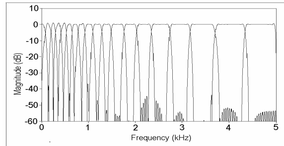
Figure 1: Spectral splitting (SS): (a) Schematic, (b) magnitude response of the comb filter pair, S.R. = 10 k Sa/s, pass band ripple < 1 dB, stop band attenuation > 30 dB, = 78 - 117 Hz transition width
